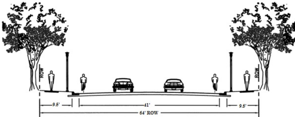
PRIMARY COLLECTOR STREET
