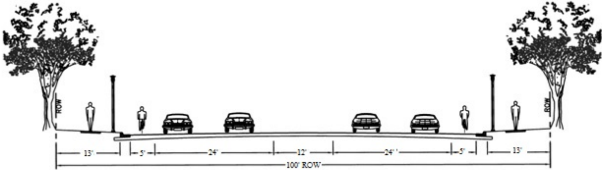
MAJOR ARTERIAL, UNDIVIDED, 5 LANES (MAU 5)
