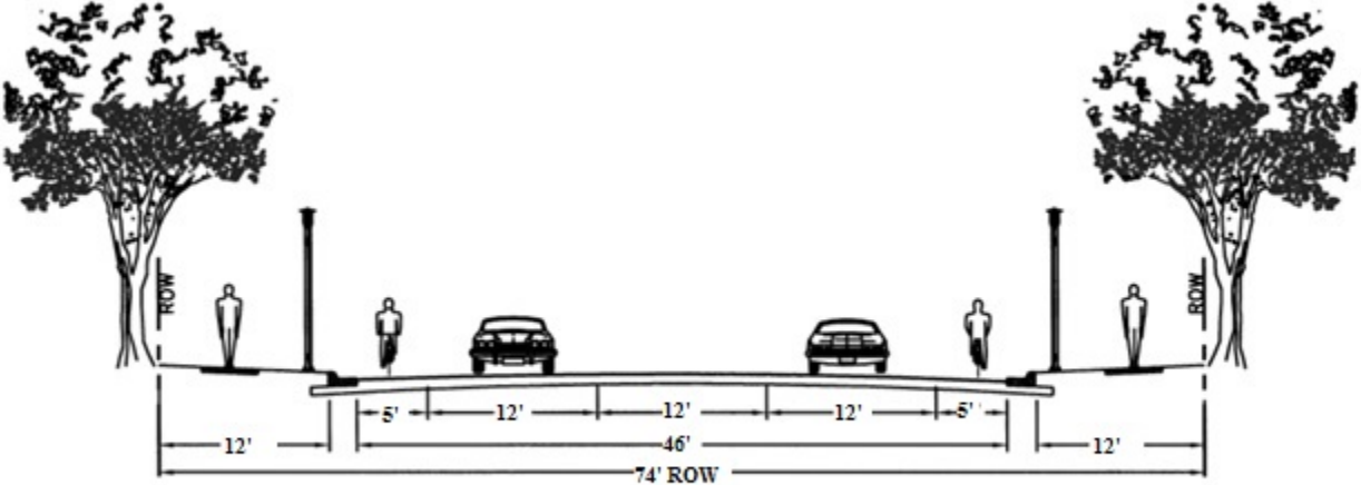
MINOR ARTERIAL, 3 LANES (MNR 3)
