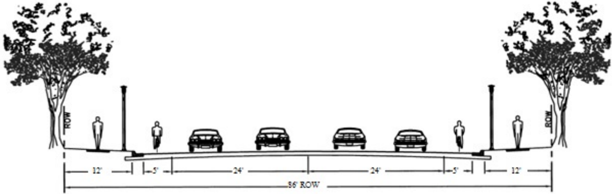
MAJOR ARTERIAL, UNDIVIDED, 4 LANES (MAU 4)
